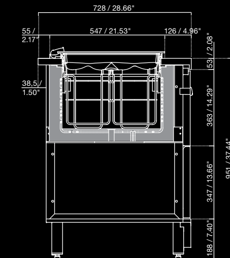
Banco PANORAMA senza riserva PANORAMA counter with one level of gelato tubs Comptoir PANORAMA sans réserve PANORAMA-Theke ohne Vorrat Mostrador PANORAMA sin reserva
